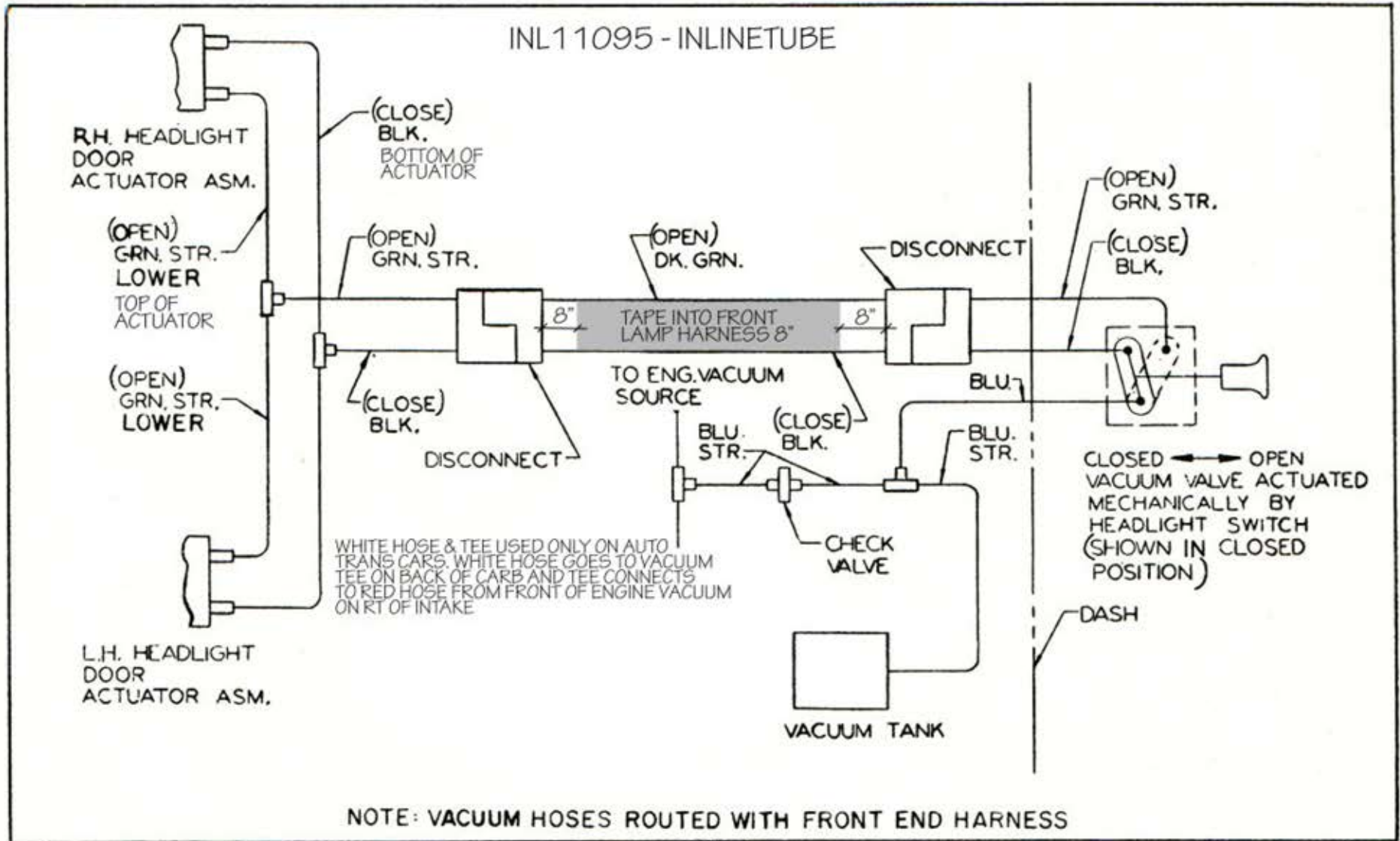
Fig. 12-41 Vacuum Operated Headlamp Door Schematic
